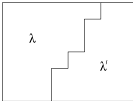
FIGURE 2. The diagrams for Poincaré dual forms on G(6, 8)
