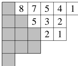
FIGURE 3. D(\lambda) , S(\lambda) and hook lengths for \lambda = (5, 3, 2)
