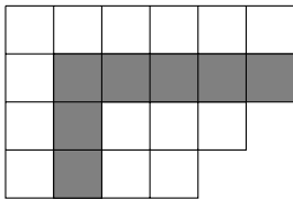
FIGURE 1. A hook in the diagram of (6, 6, 5, 4)
