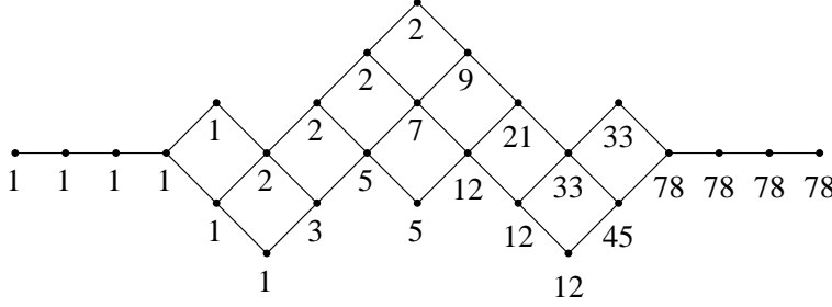
FIGURE 4. The poset of Schubert forms for E_6/(SO(10) \cdot SO(2))
