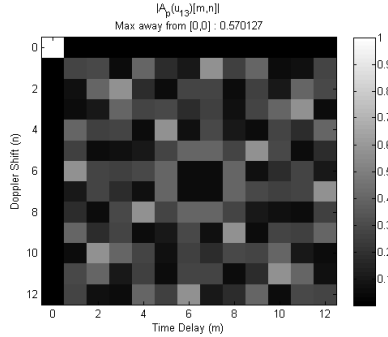
FIGURE 2. A_p(u_p) for p = 13
