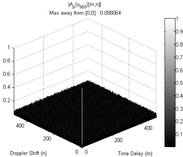
FIGURE 3. A_p(u_p) for p = 503
