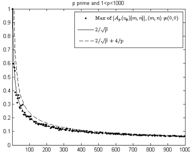
FIGURE 1. p and \max\{|A_p(u_p)[m, n]| : (m, n) \neq (0, 0)\}
