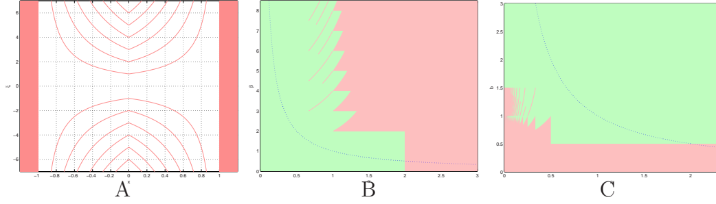
Fig. 1. A: Zero set of V_{1_{[0,1]}} \mathbf{1}_{[0,1]} (dark). B: Set containing all pairs (\alpha, \beta) , \alpha, \beta > 0 such that P_{\alpha\mathbb{Z} \times \beta\mathbb{Z}} |V_g|^2 has a root (dark). We include as reference the curve \alpha\beta = 1 (dashed). C: Set containing all pairs (a, b) , a, b > 0 such that \{\rho(an, bm)P_g\}_{n,m \in \mathbb{Z}} is not a Riesz basis in HS(\mathbb{R}) (dark). The curve ab = 1 is included (dashed).
