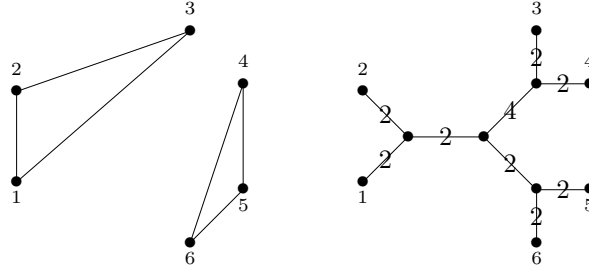
FIGURE 3. A graph on the leaves of a trivalent tree and its associated weighting.
