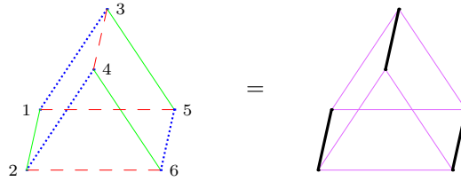
FIGURE 6. A generalized Segre relation on six points. Here U_G = \{1, 2\} , U_R = \{3, 4\} and U_B = \{5, 6\} . This is equal to the image of the usual Segre cubic relation in I_L/Q_L .
