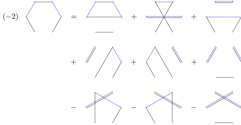
FIGURE 7. A graphical identity on 6 points. More accurately, this should be regarded as a family of identities between various tensors Y_\Gamma \otimes Y_\Delta in V_L^{\otimes 2} for any L ; we have only drawn the edges on each side which are different.
