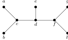
FIGURE 1. A trivalent tree. Vertices c, d and f are trinodes; the rest are leaves. The vertices a and b form a matched pair, as do the vertices g and h . The tree is not matched because e does not belong to a matched pair.
