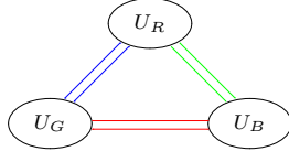
FIGURE 5. Schematic presentation of a generalized Segre datum.
