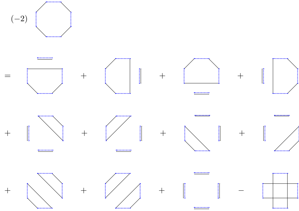
FIGURE 9. A graphical identity. The blue edges here are not relevant to the identity: they are just drawn to emphasize the disconnectedness of the graphs on the right side. Thus this is a linear relation between Y_\Gamma 's where the \Gamma are matchings on 8 points. This identity can be obtained by applying the procedure of Proposition 6.9 to the term on the left side, or by applying the straightening algorithm to the final term on the right side.
