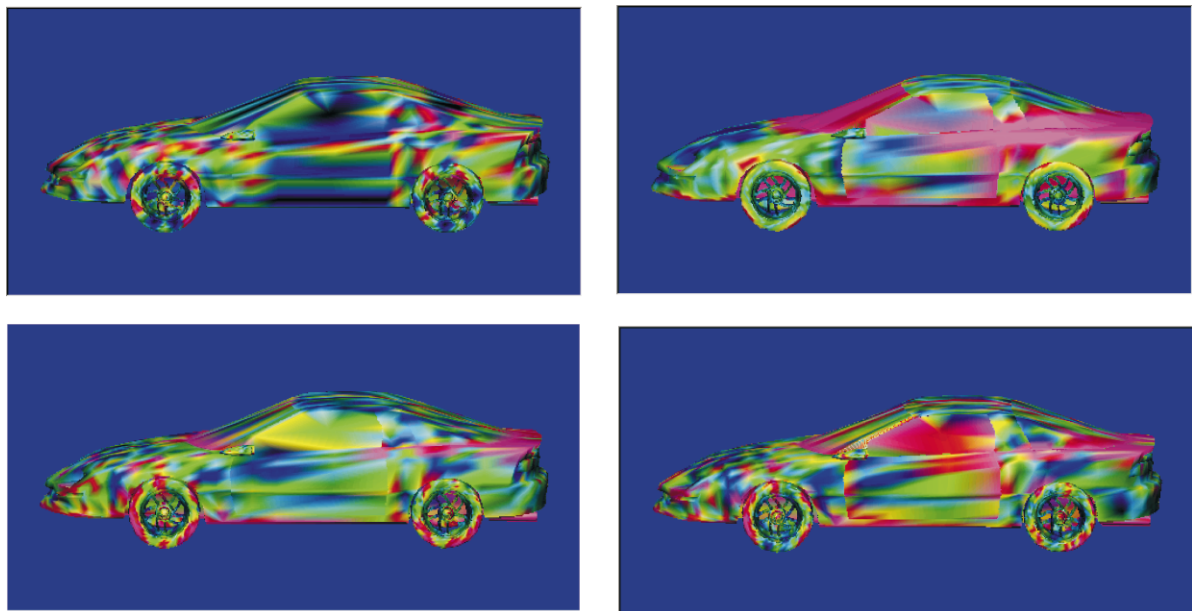
Fig. 4. The color plot of the single resolution approximation errors for the four different filters: Zeroth Order Filter (upper left); Gaussian Smoothing (upper right); LS first order (lower left) and LS third order (lower right).
