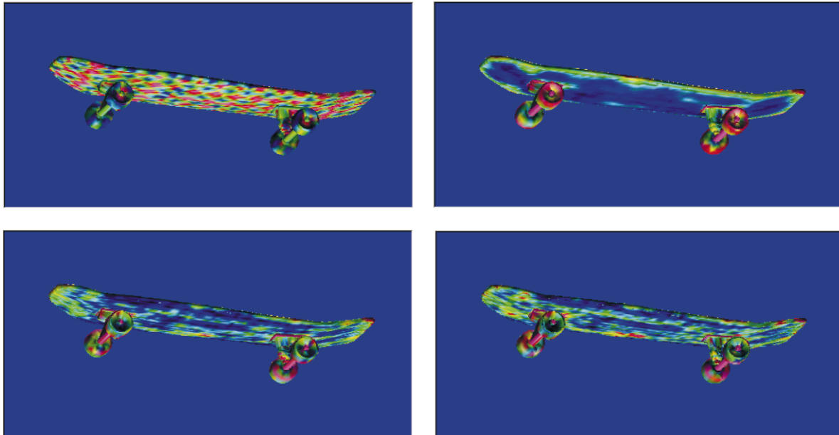
Fig. 12. The color plot of the single resolution approximation errors for the four different filters: Zeroth Order Filter (upper left); Gaussian Smoothing (upper right); LS first order (lower left) and LS third order (lower right).
