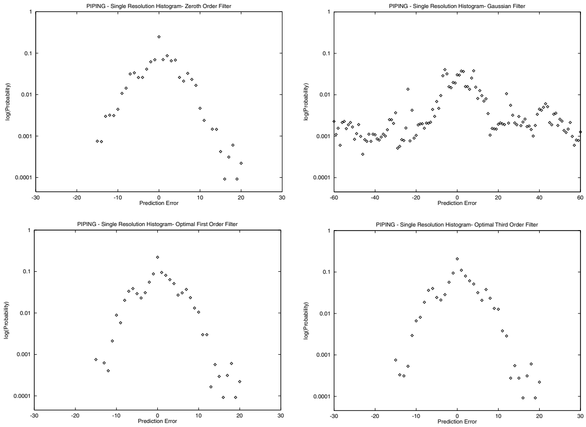
Fig. 15. Semilog histograms of the prediction errors associated to the four filters for the Single Resolution scheme applied to the mesh rendered in Fig. 13.
