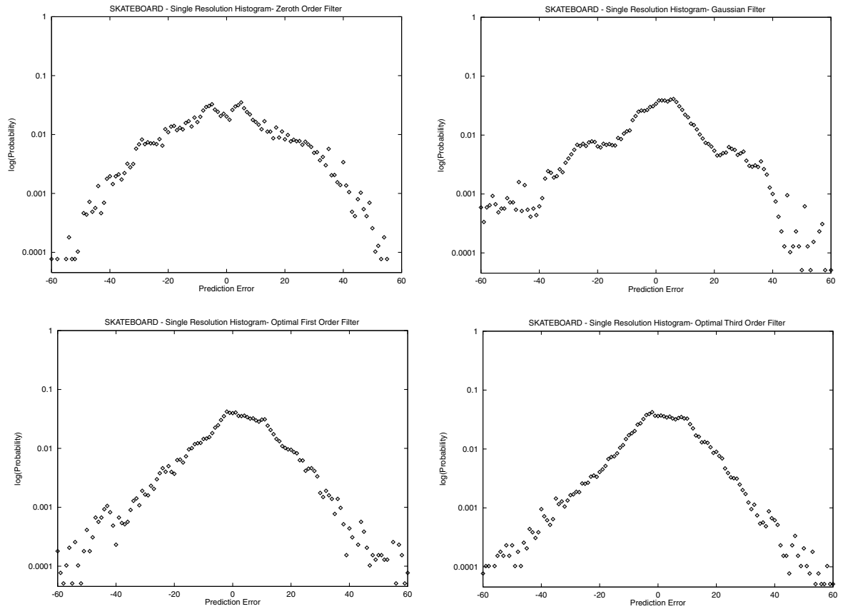
Fig. 11. Semilog histograms of the prediction errors associated to the four filters for the Single Resolution scheme applied to the mesh rendered in Fig. 9.
