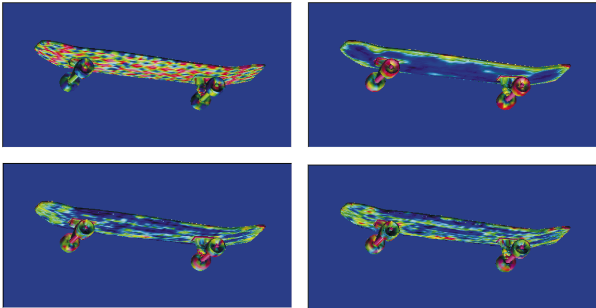
Fig. 16. The color plot of the single resolution approximation errors for the four different filters: Zeroth Order Filter (upper left); Gaussian Smoothing (upper right); LS first order (lower left) and LS third order (lower right).
