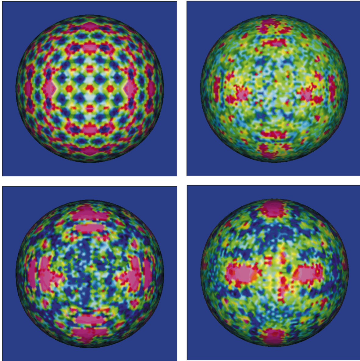
Fig. 20. The color plot of the single resolution approximation errors for the four different filters: Zeroth Order Filter (upper left); Gaussian Smoothing (upper right); LS first order (lower left) and LS third order (lower right).
