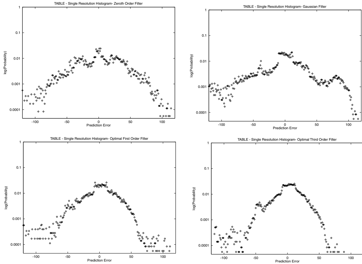
Fig. 7. Semilog histograms of the prediction errors associated to the four filters for the Single Resolution scheme applied to the round table rendered in Fig. 5.
