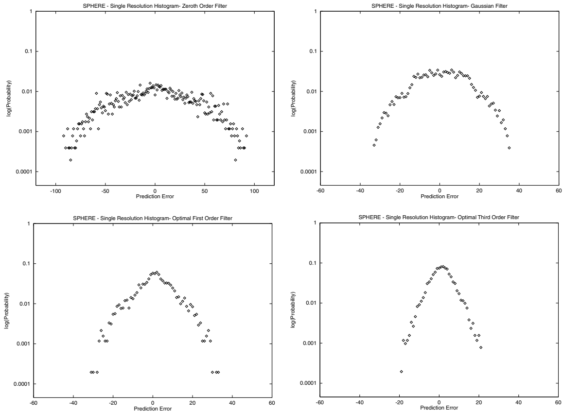
Fig. 19. Semilog histograms of the prediction errors associated to the four filters for the Single Resolution scheme applied to the sphere mesh rendered in Fig. 17.
