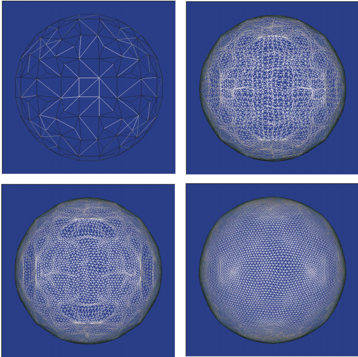
Fig. 18. The sphere at the finest resolution level when no difference is used and the filtering is performed by: the Zeroth Order Filter (top left); the Gaussian Smoother (top right); the least squares filter of order 1 (bottom left) and the least squares filter of order 3 (bottom right).
