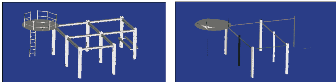
Fig. 13. The piping mesh at the finest resolution (left) and the coarsest resolution (right) after seven levels of reduction.
