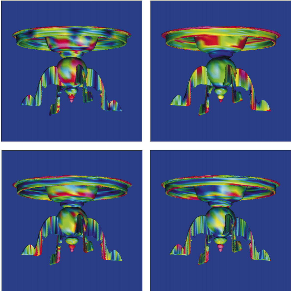
Fig. 8. The color plot of the single resolution approximation errors for the four different filters: Zeroth Order Filter (upper left); Gaussian Smoothing (upper right); LS first order (lower left) and LS third order (lower right).
