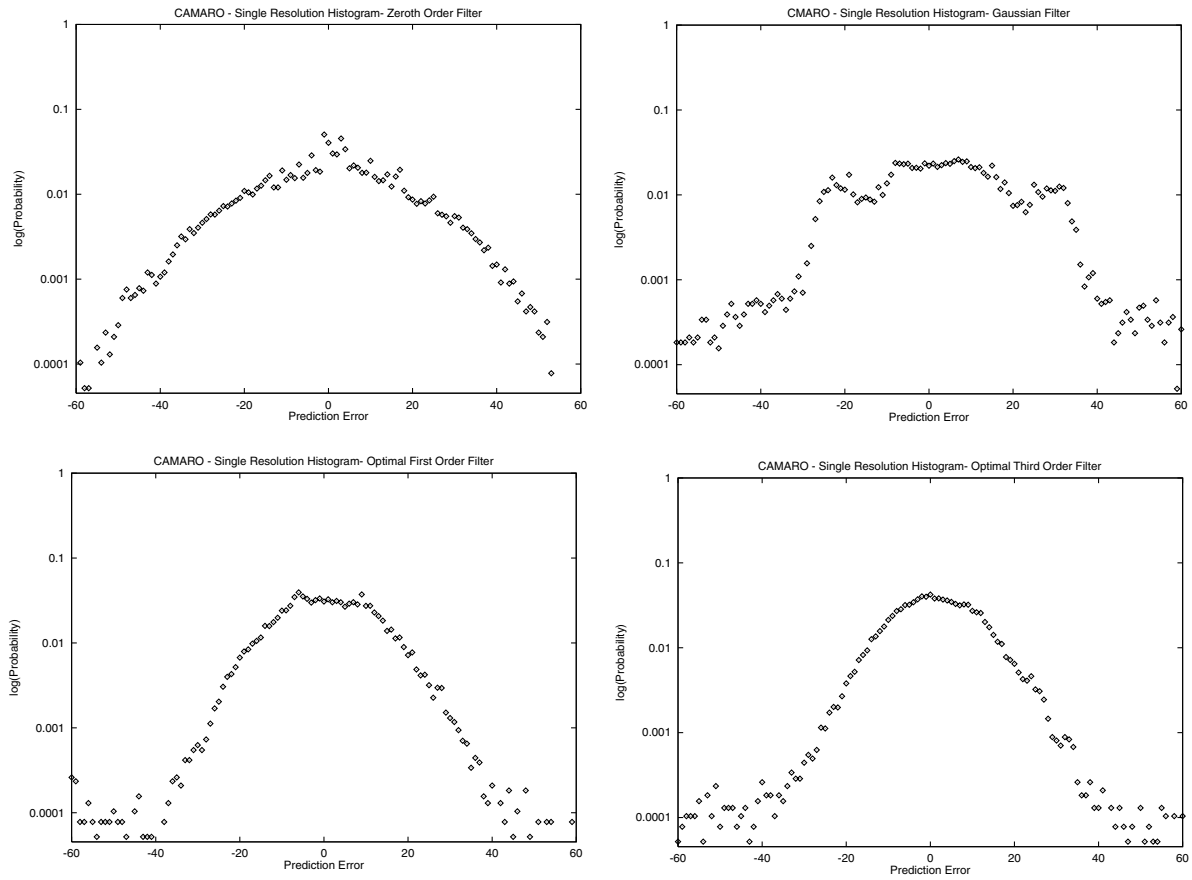
Fig. 3. Semilog histograms of the prediction errors associated to the four filters for the Single Resolution scheme applied to the car mesh rendered in Fig. 1.
