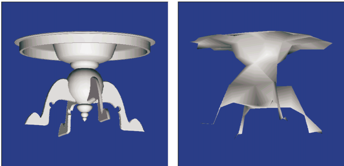
Fig. 5. The round table mesh at the finest resolution (left) and the coarsest resolution (right) after seven levels of reduction.
